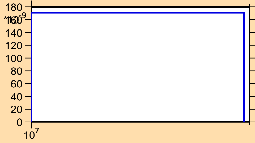
\sigma vs. E for ^{135}\text{Gd}(n,2n\alpha)
