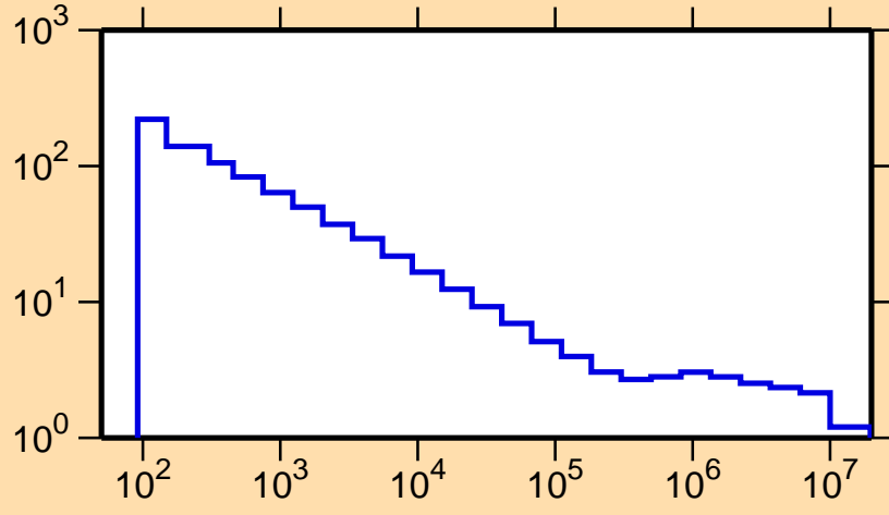
\sigma vs. E for ^{135}\text{Gd}(n,\text{nonel.})
