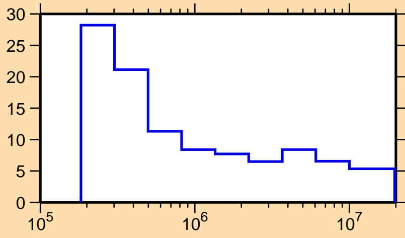
\Delta\sigma/\sigma vs. E for ^{135}\text{Gd}(n,\text{tot.})
