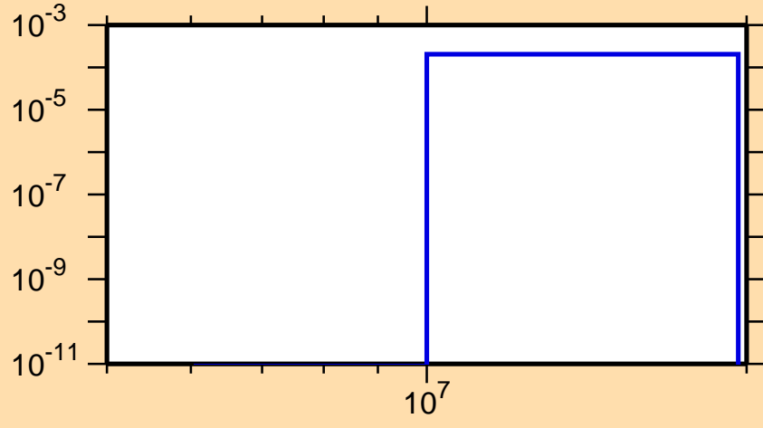
\sigma vs. E for ^{135}\text{Gd}(n,\text{pt})
