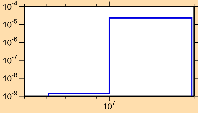
\sigma vs. E for ^{135}\text{Gd} (mt 45)
