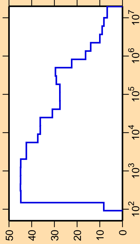
\Delta\sigma/\sigma vs. E for ^{135}\text{Gd}(n,\text{nonel.})
