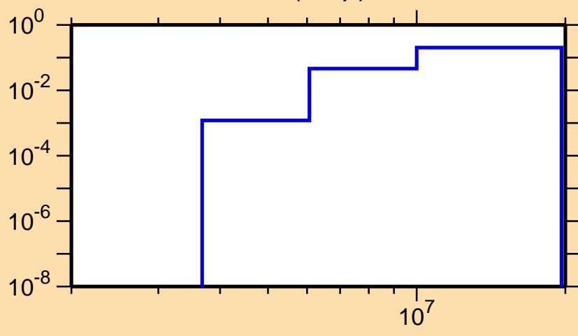
\sigma vs. E for ^{135}\text{Gd}(n,np)
