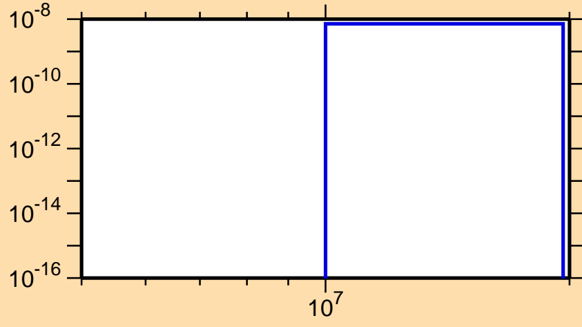
\sigma vs. E for ^{135}\text{Gd} (mt 34)
