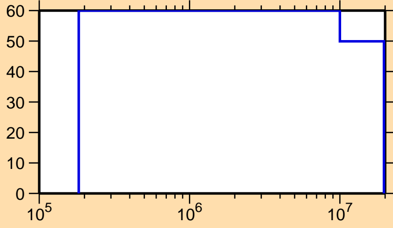
\Delta\sigma/\sigma vs. E for ^{135}\text{Gd}(n,n\text{cont.})
