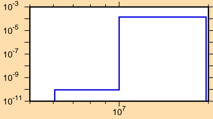
\sigma vs. E for ^{135}\text{Gd}(n,t)
