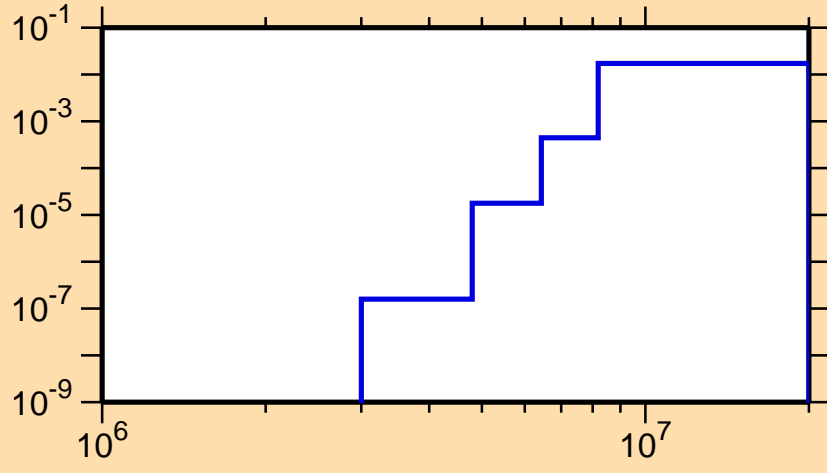
\sigma vs. E for ^{135}\text{Gd}(n,d)
