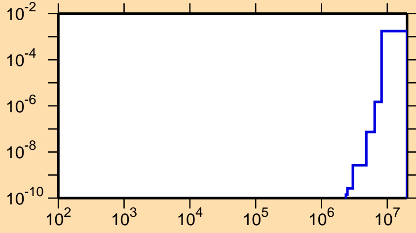
\sigma vs. E for ^{135}\text{Gd}(n,\text{He3})
