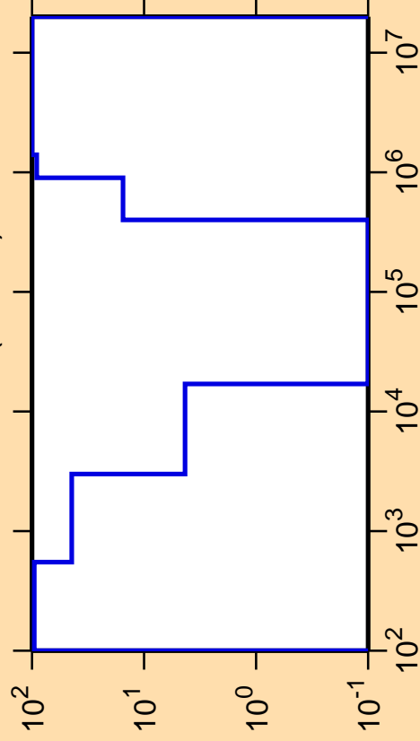
\Delta\sigma/\sigma vs. E for ^{135}\text{Gd}(n,\text{He3})
