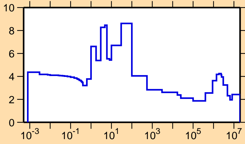
\sigma vs. E for ^{135}\text{Gd}(n,\text{el.})
