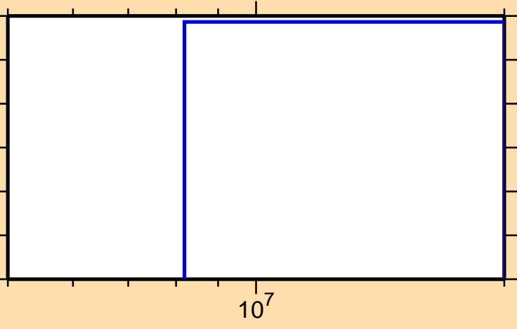
\sigma vs. E for ^{135}\text{Gd} (mt 34)
