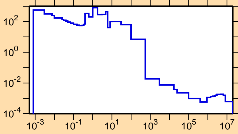
\sigma vs. E for ^{135}\text{Gd}(n,\gamma)
