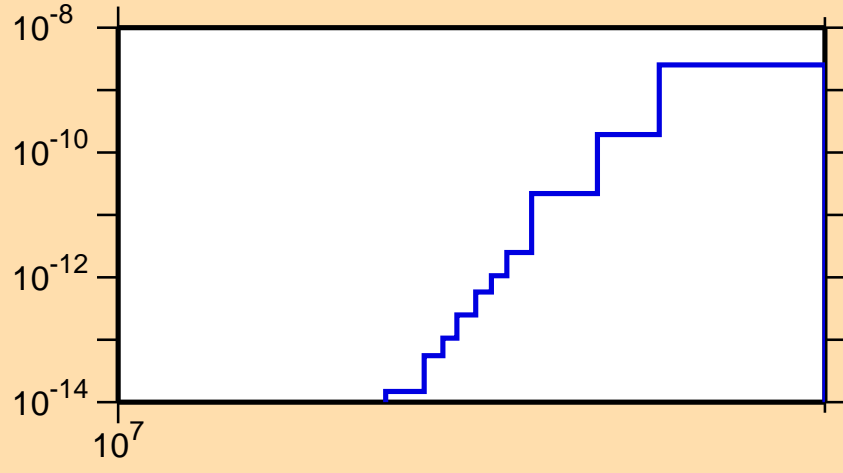
\sigma vs. E for ^{136}\text{Gd} (mt 34)
