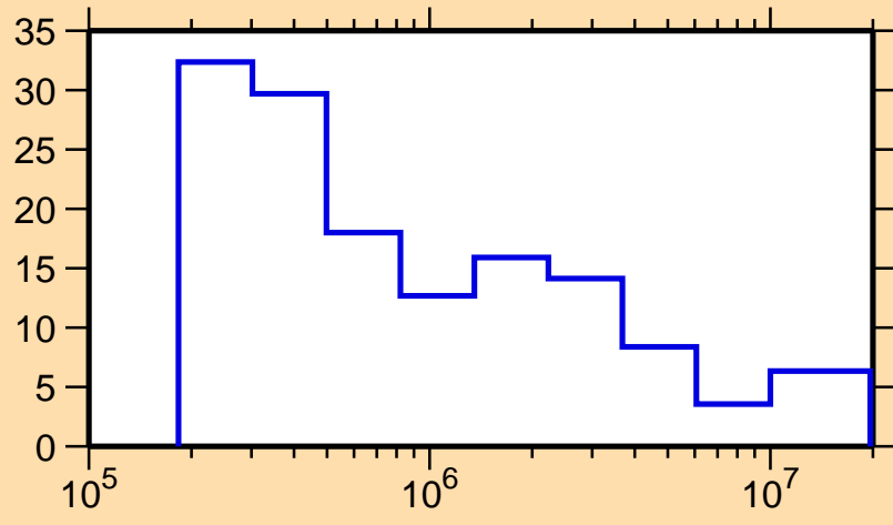
\Delta\sigma/\sigma vs. E for ^{136}\text{Gd}(n,\text{tot.})
