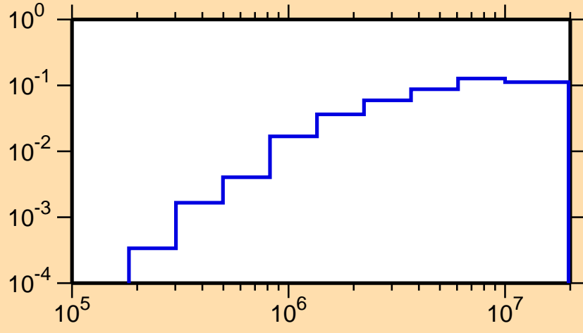
\sigma vs. E for ^{136}\text{Gd}(n,n\text{cont.})
