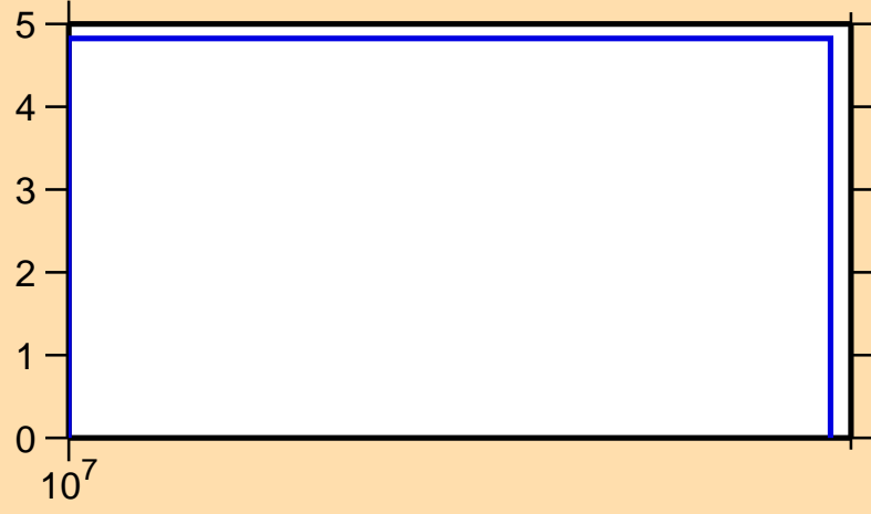
\Delta\sigma/\sigma vs. E for ^{136}\text{Gd}(n,\text{nonel.})
