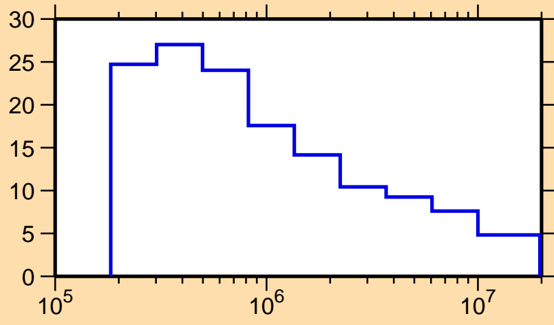
\Delta\sigma/\sigma vs. E for ^{136}\text{Gd}(n,n\text{onel.})
