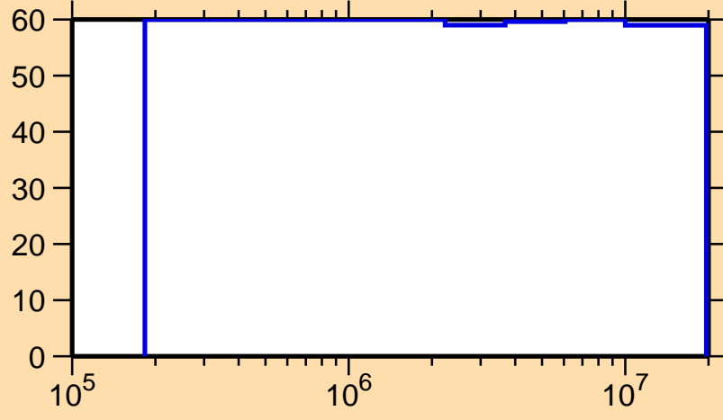
\Delta\sigma/\sigma vs. E for ^{136}\text{Gd}(n,n\text{cont.})
