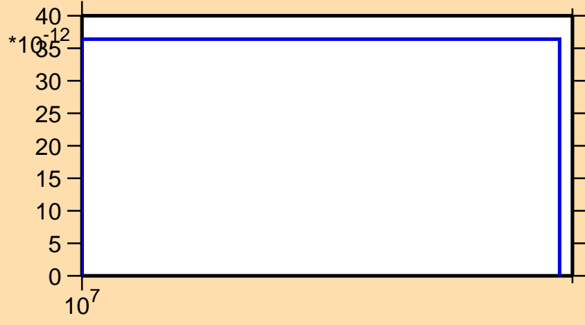
\sigma vs. E for ^{136}\text{Gd} (mt 34)
