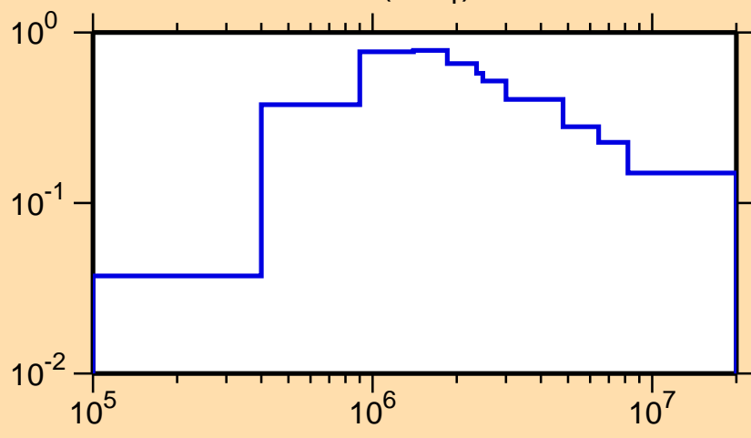
\sigma vs. E for ^{136}\text{Gd}(n,n_1)
