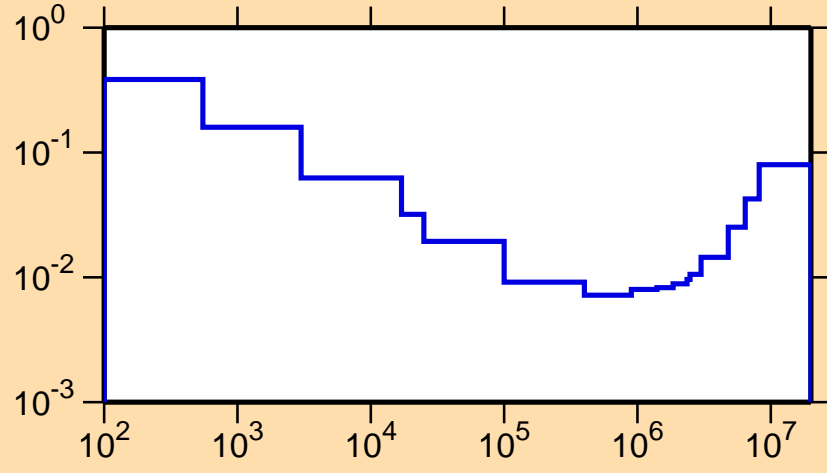
\sigma vs. E for ^{136}\text{Gd}(n,\alpha)
