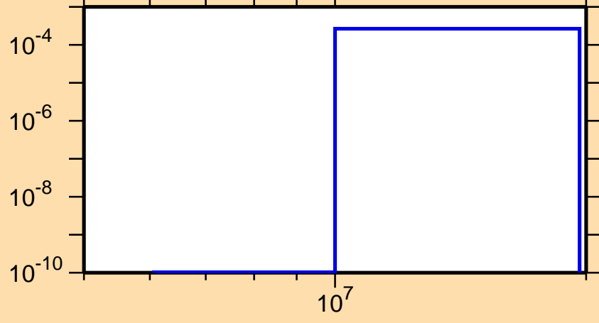
\sigma vs. E for ^{137}\text{Gd}(n,t)
