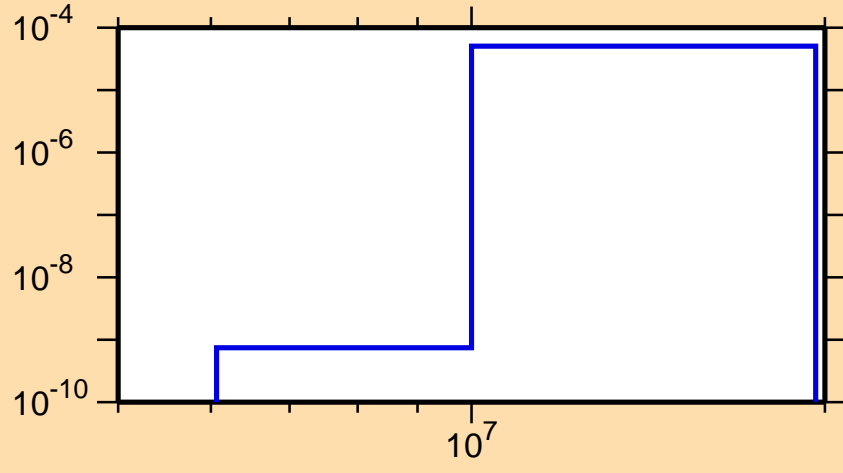
\sigma vs. E for ^{137}\text{Gd} (mt 45)
