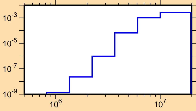
\sigma vs. E for ^{137}\text{Gd}(n,n\alpha)
