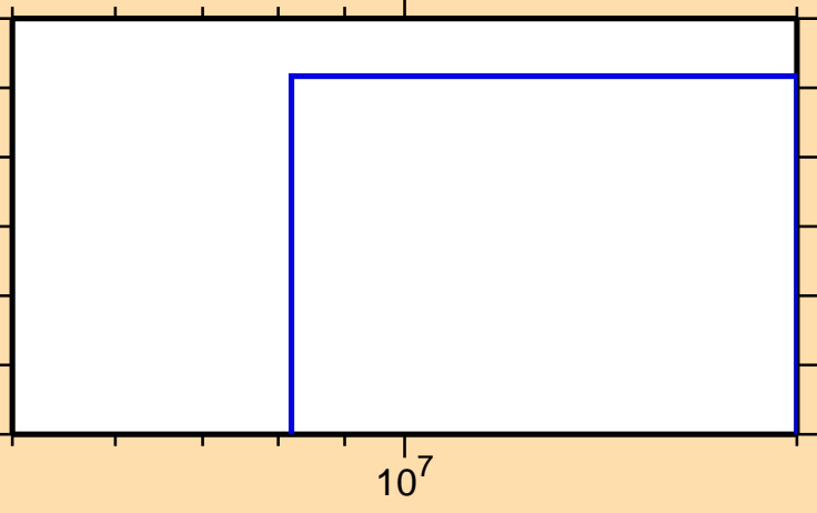
\sigma vs. E for ^{137}\text{Gd}(n,\text{nd})
