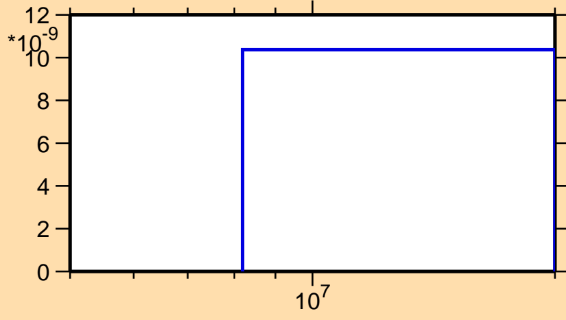
\sigma vs. E for ^{137}\text{Gd} (mt 34)
