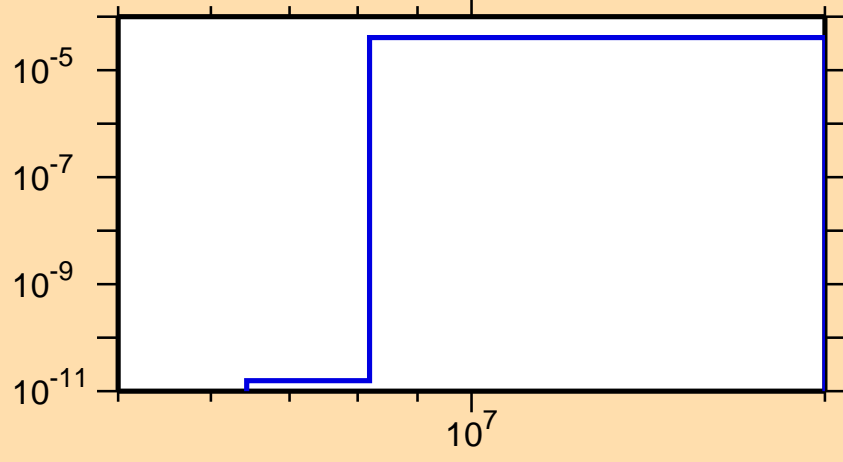
\sigma vs. E for ^{137}\text{Gd} (mt 45)
