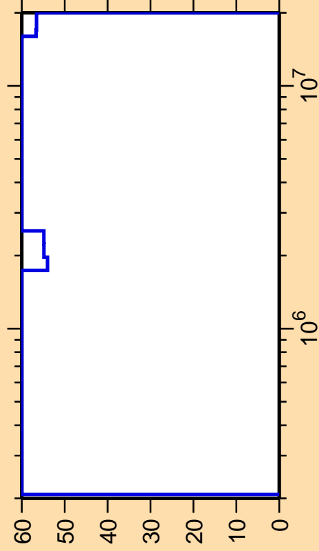
\Delta\sigma/\sigma vs. E for ^{138}\text{Gd}(n,\text{inel.})
