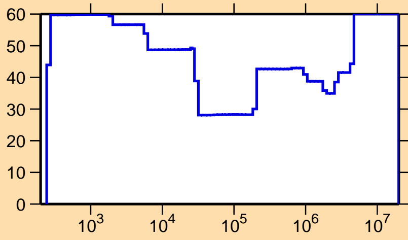
\Delta\sigma/\sigma vs. E for ^{138}\text{Gd}(n,p)
