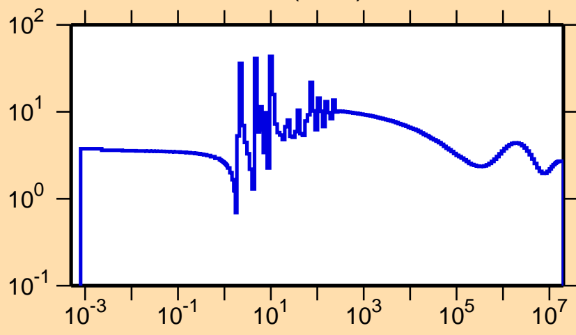
\sigma vs. E for ^{138}\text{Gd}(n,\text{el.})
