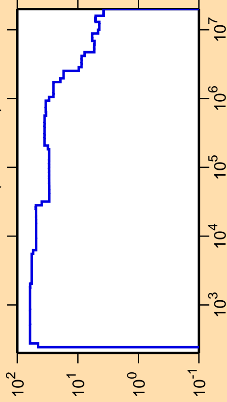
\Delta\sigma/\sigma vs. E for ^{138}\text{Gd}(n,\text{nonel.})
