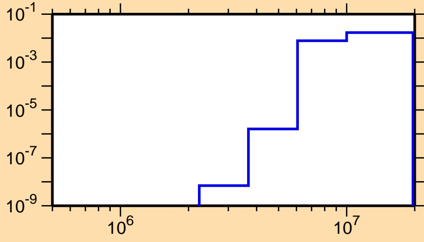
\sigma vs. E for ^{138}\text{Gd}(n,n\alpha)
