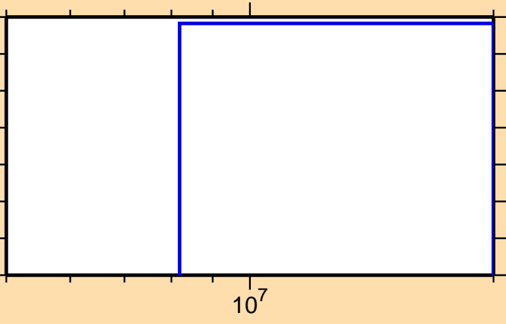
\sigma vs. E for ^{139}\text{Gd}(n,2np)
