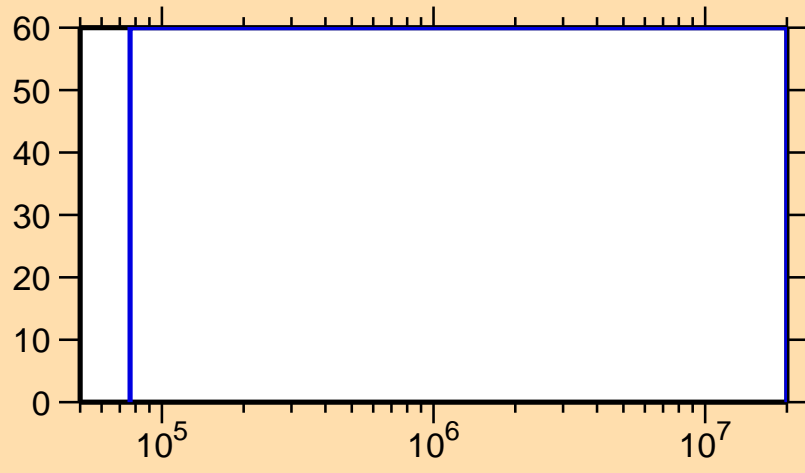
\Delta\sigma/\sigma vs. E for ^{139}\text{Gd}(n,n\text{cont.})
