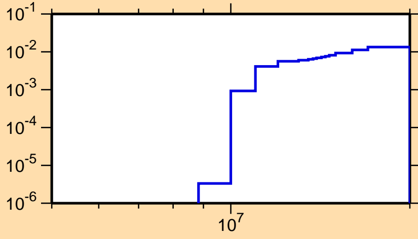
\sigma vs. E for ^{139}\text{Gd}(n,2n)
