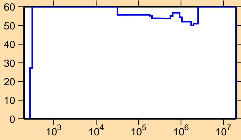
\Delta\sigma/\sigma vs. E for ^{139}\text{Gd}(n,p)
