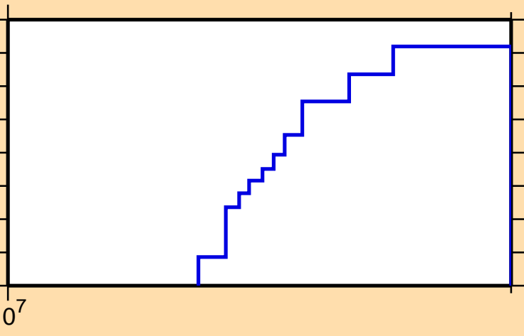
\sigma vs. E for ^{139}\text{Gd}(n,\text{nd})
