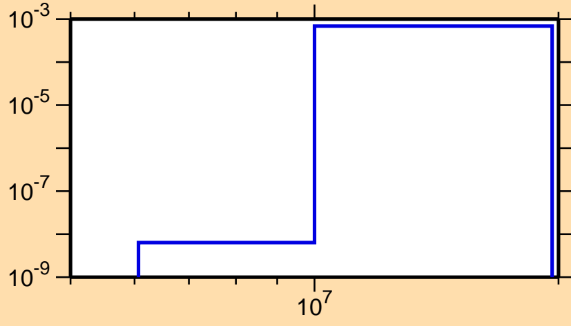
\sigma vs. E for ^{139}\text{Gd}(n,\text{pd})
