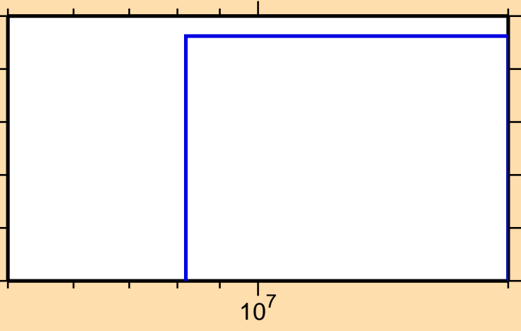
\sigma vs. E for ^{139}\text{Gd} (mt 34)
