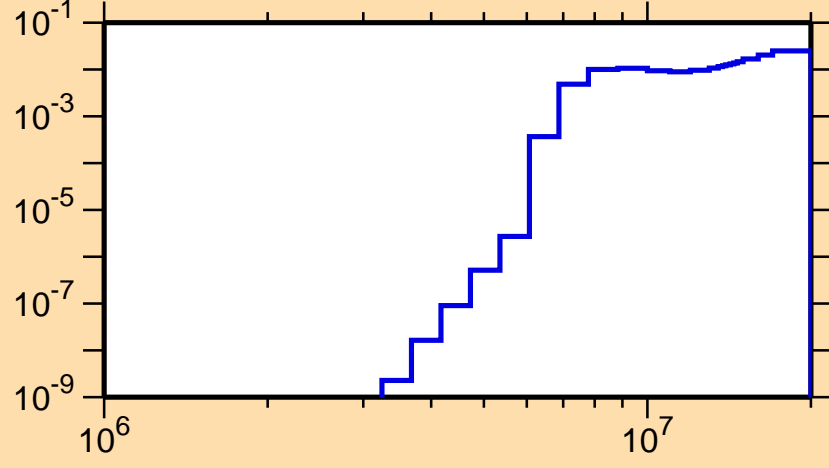
\sigma vs. E for ^{140}\text{Gd}(n,n\alpha)
