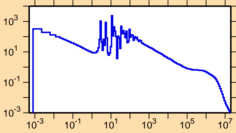
\sigma vs. E for ^{140}\text{Gd}(n,\gamma)
