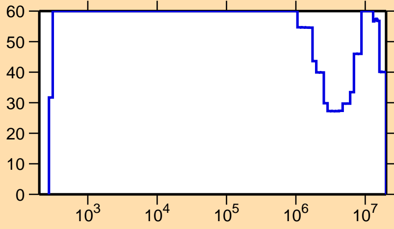
\Delta\sigma/\sigma vs. E for ^{140}\text{Gd}(n,p)
