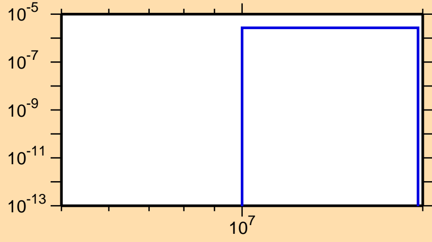
\sigma vs. E for ^{140}\text{Gd} (mt 45)
