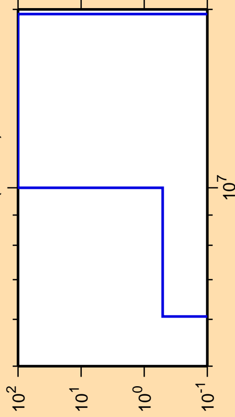
\Delta\sigma/\sigma vs. E for ^{140}\text{Gd} (mt 45)
