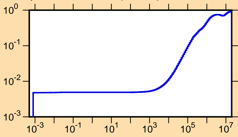
\mu vs. E for ^{141}\text{Gd}(\text{mt251})
