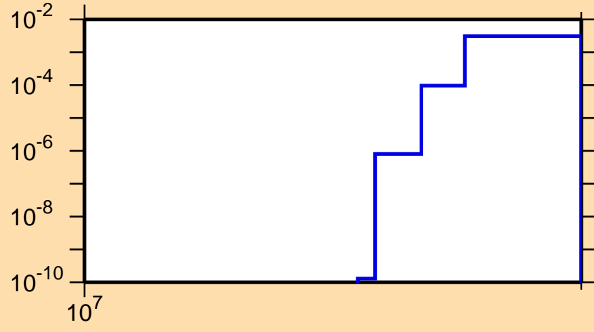
\sigma vs. E for ^{141}\text{Gd}(n,2np)
