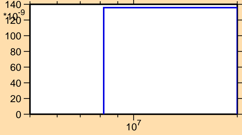
\sigma vs. E for ^{141}\text{Gd}(n,nd)
