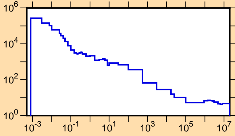
\sigma vs. E for ^{141}\text{Gd}(n,\text{tot.})
