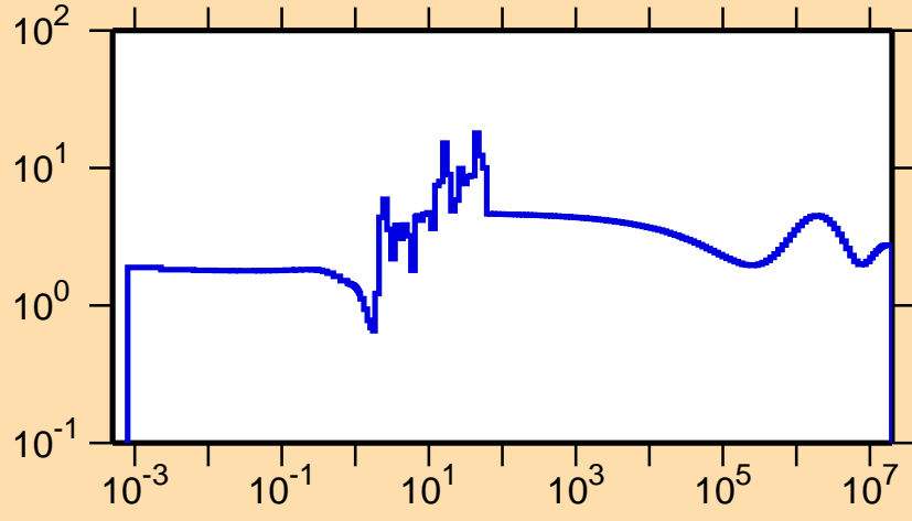
\sigma vs. E for ^{141}\text{Gd}(n,\text{el.})
