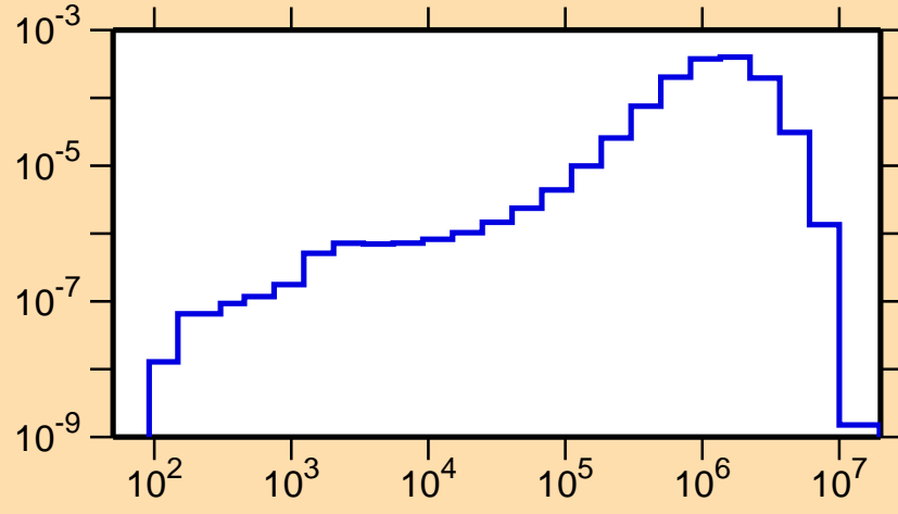
\sigma vs. E for ^{141}\text{Gd}(n,n_1)
