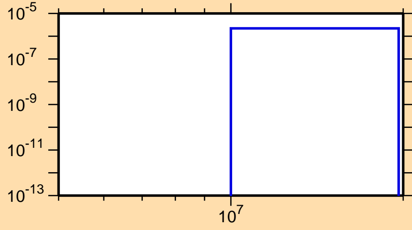
\sigma vs. E for ^{141}\text{Gd} (mt 45)
