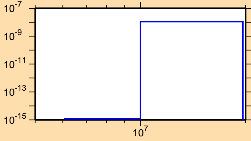
\sigma vs. E for ^{141}\text{Gd}(\text{mt117})
