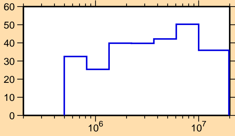
\Delta\sigma/\sigma vs. E for ^{141}\text{Gd}(n,el.)
