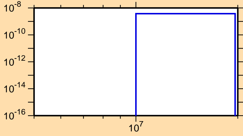
\sigma vs. E for ^{142}\text{Gd}(\text{mt117})
