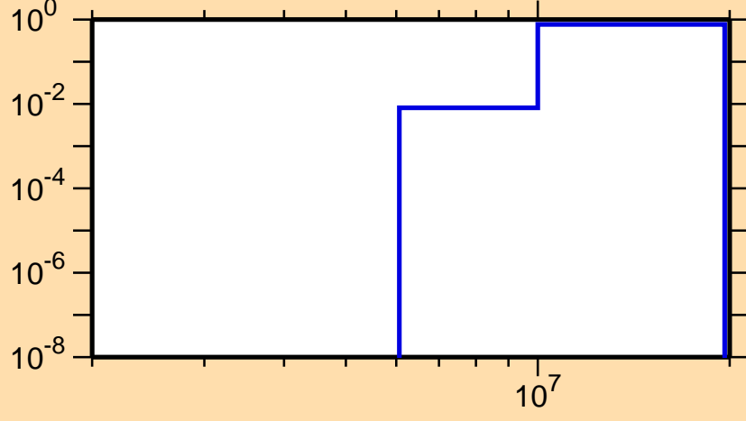
\sigma vs. E for ^{142}\text{Gd}(n,np)
