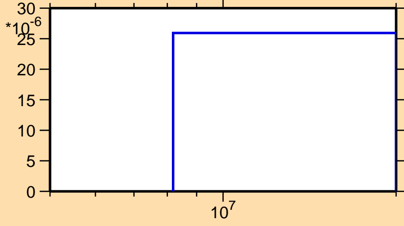
\sigma vs. E for ^{142}\text{Gd}(n,t)
