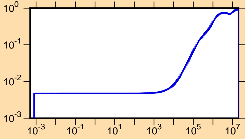
\mu vs. E for ^{143}\text{Gd}(\text{mt251})
