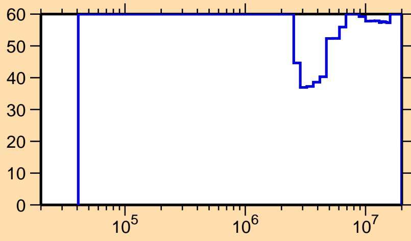
\Delta\sigma/\sigma vs. E for ^{143}\text{Gd}(n,n_1)
