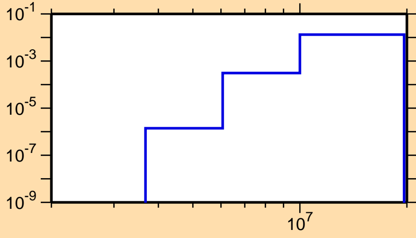
\sigma vs. E for ^{143}\text{Gd}(n,n\alpha)
