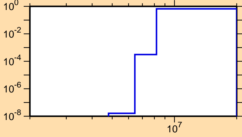
\sigma vs. E for ^{143}\text{Gd}(n,np)
