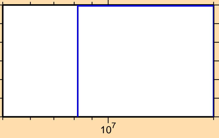
\sigma vs. E for ^{143}\text{Gd}(n,t)
