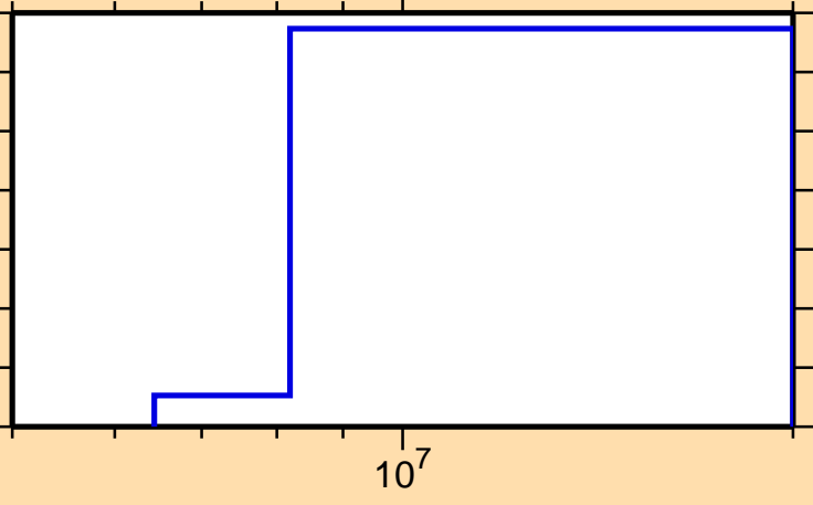
\sigma vs. E for ^{143}\text{Gd}(n,\text{He3})
