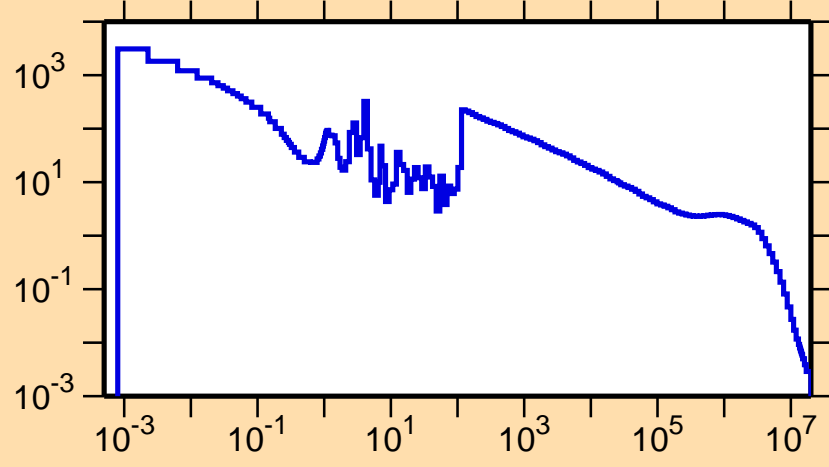
\sigma vs. E for ^{143}\text{Gd}(n,\gamma)
