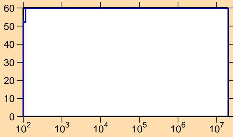
\Delta\sigma/\sigma vs. E for ^{143}\text{Gd}(n,\gamma)
