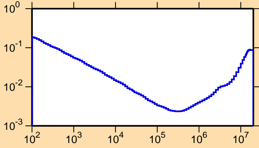
\sigma vs. E for ^{143}\text{Gd}(n,\alpha)
