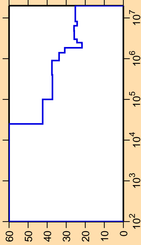
\Delta\sigma/\sigma vs. E for ^{143}\text{Gd}(n,\text{nonel.})
