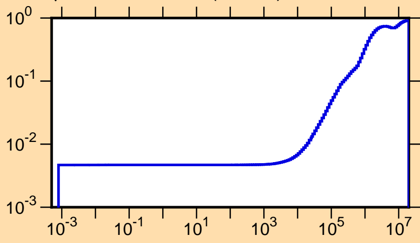
\mu vs. E for ^{144}\text{Gd}(\text{mt251})
