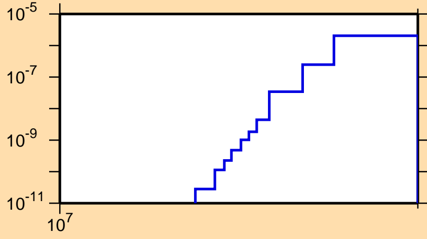
\sigma vs. E for ^{144}\text{Gd} (mt 45)
