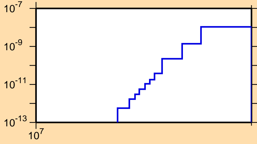
\sigma vs. E for ^{144}\text{Gd}(\text{mt117})
