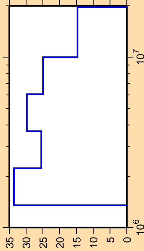
\Delta\sigma/\sigma vs. E for ^{144}\text{Gd}(n,n_4)
