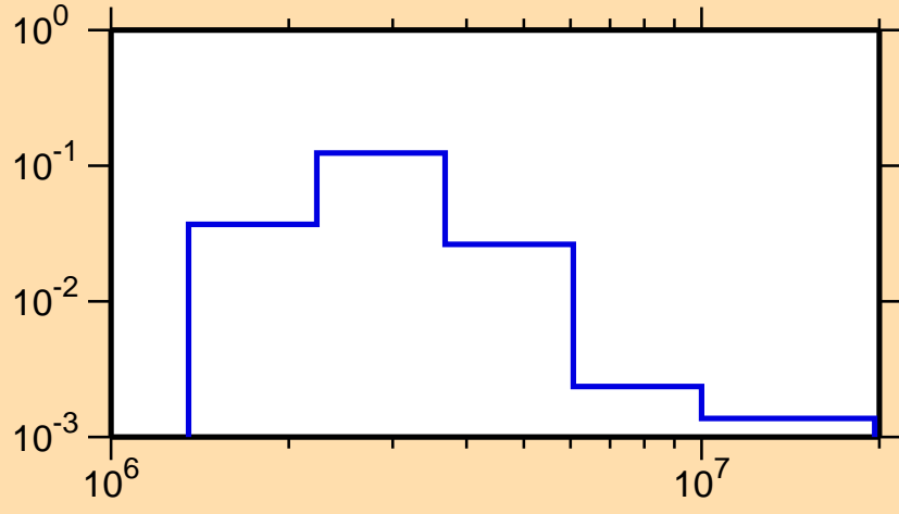
\sigma vs. E for ^{144}\text{Gd}(n,n_4)
