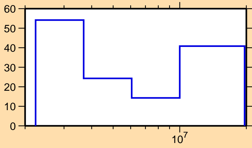
\Delta\sigma/\sigma vs. E for ^{144}\text{Gd}(n,n\text{cont.})
