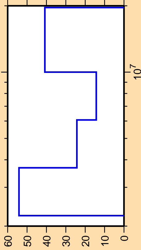
\Delta\sigma/\sigma vs. E for ^{144}\text{Gd}(n,n\text{cont.})
