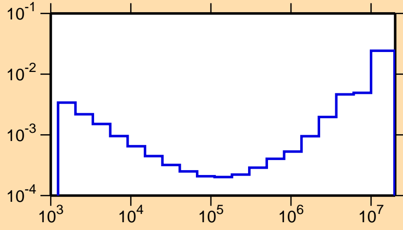
\sigma vs. E for ^{144}\text{Gd}(n,\alpha)
