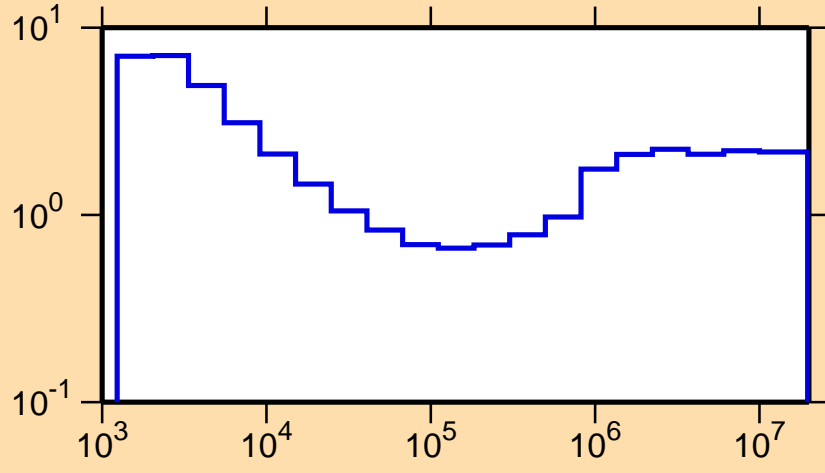
\sigma vs. E for ^{144}\text{Gd}(n,\text{nonel.})
