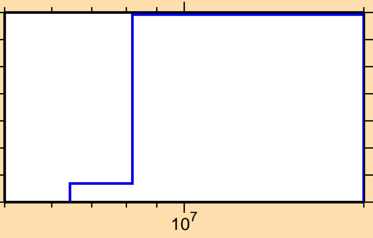
\sigma vs. E for ^{144}\text{Gd}(n,\text{He3})
