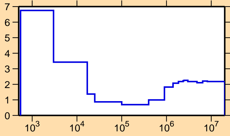
\sigma vs. E for ^{144}\text{Gd}(n,\text{nonel.})
