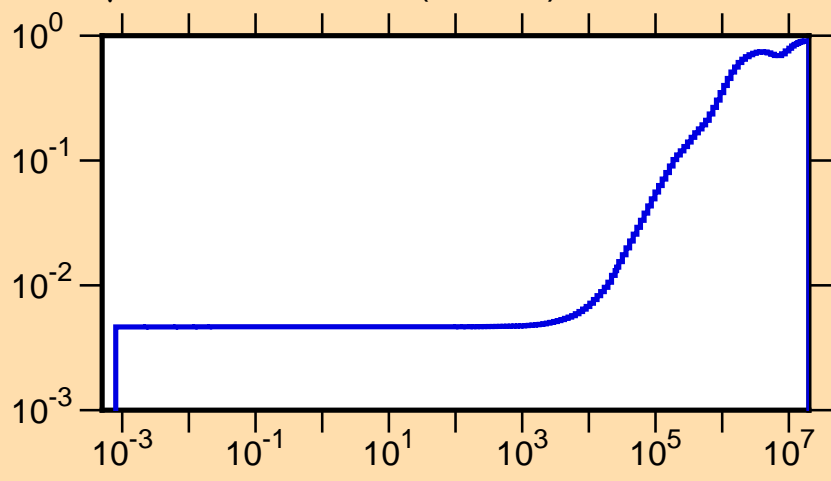
\mu vs. E for ^{145}\text{Gd}(\text{mt251})
