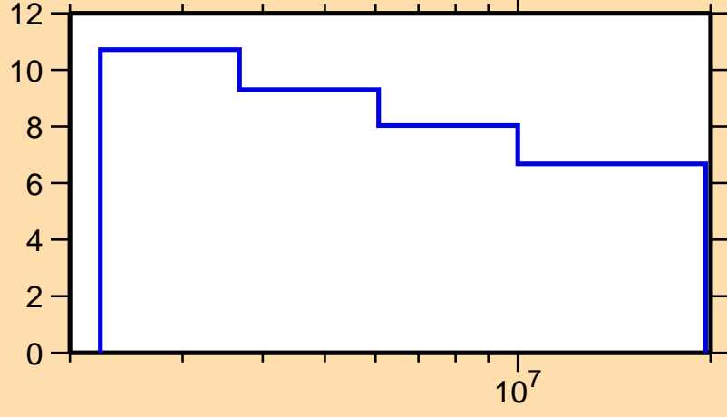
\Delta\sigma/\sigma vs. E for ^{145}\text{Gd}(n,n\text{onel.})
