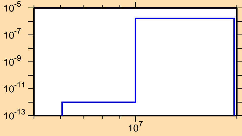
\sigma vs. E for ^{145}\text{Gd}(n,\text{He3})
