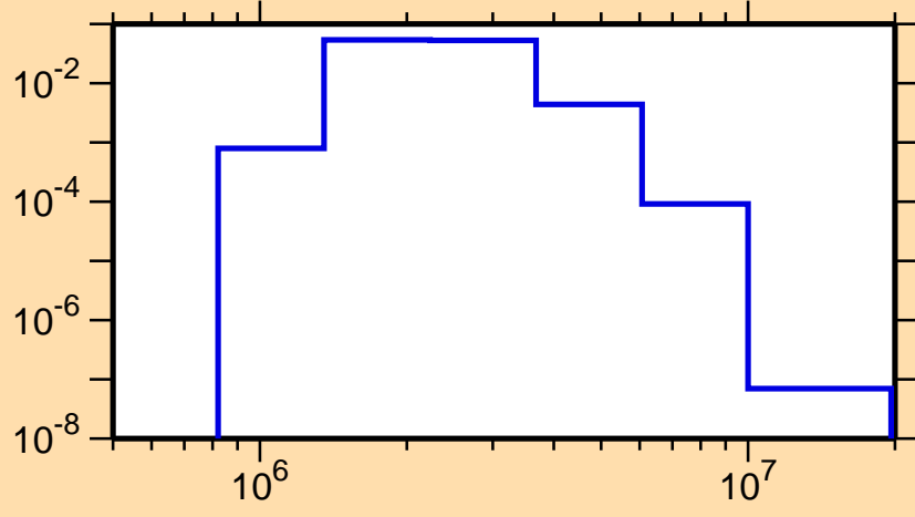
\sigma vs. E for ^{145}\text{Gd}(n,n_4)
