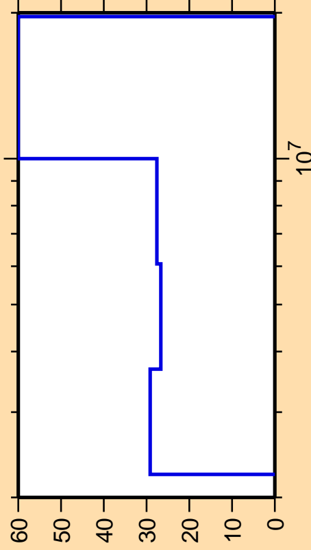
\Delta\sigma/\sigma vs. E for ^{145}\text{Gd}(n,n\text{cont.})
