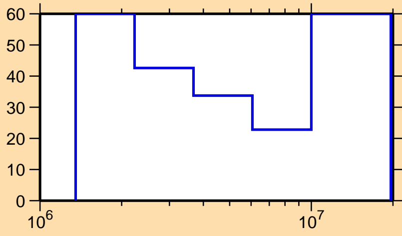
\Delta\sigma/\sigma vs. E for ^{145}\text{Gd}(n,n\text{cont.})
