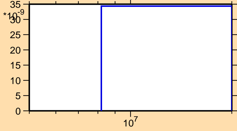
\sigma vs. E for ^{145}\text{Gd}(n,nd)
