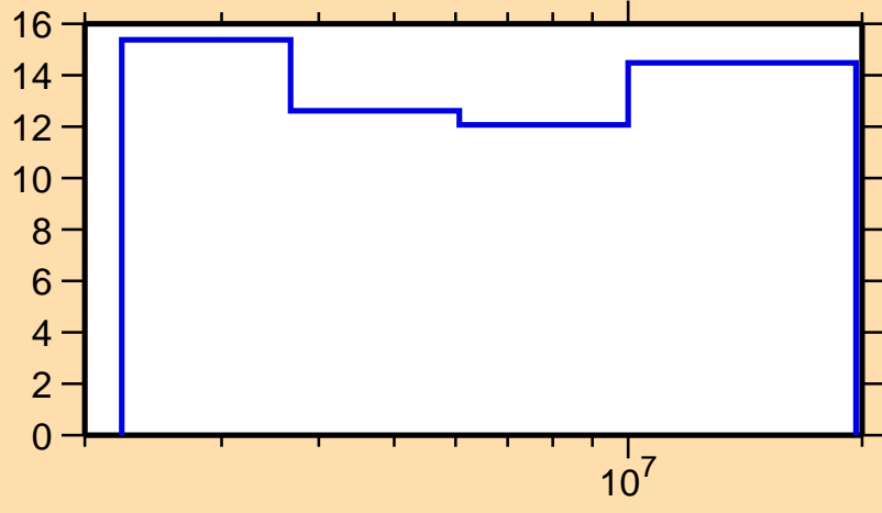
\Delta\sigma/\sigma vs. E for ^{146}\text{Gd}(n,n\text{onel.})
