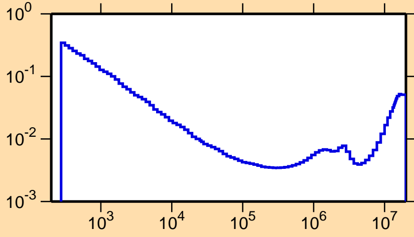
\sigma vs. E for ^{147}\text{Gd}(n,\alpha)
