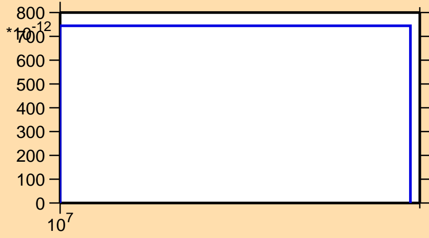
\sigma vs. E for ^{147}\text{Gd} (mt 45)
