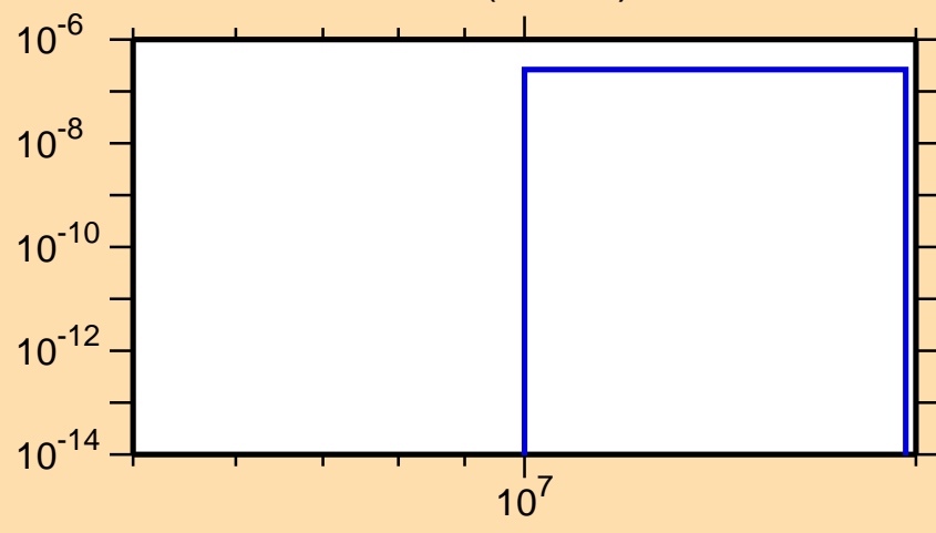
\sigma vs. E for ^{147}\text{Gd}(n,2n\alpha)
