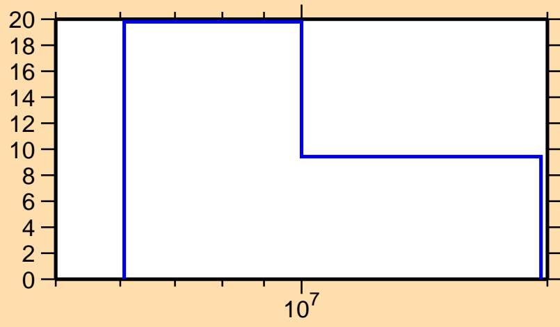
\Delta\sigma/\sigma vs. E for ^{147}\text{Gd}(n,\text{tot.})
