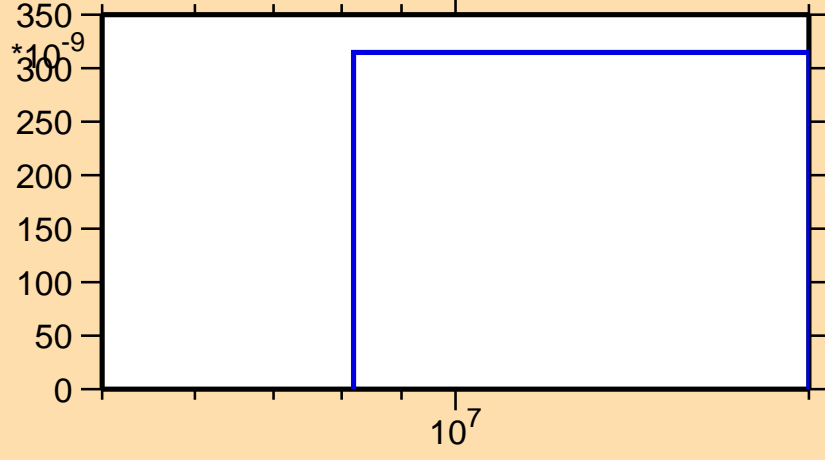
\sigma vs. E for ^{147}\text{Gd}(n,nd)
