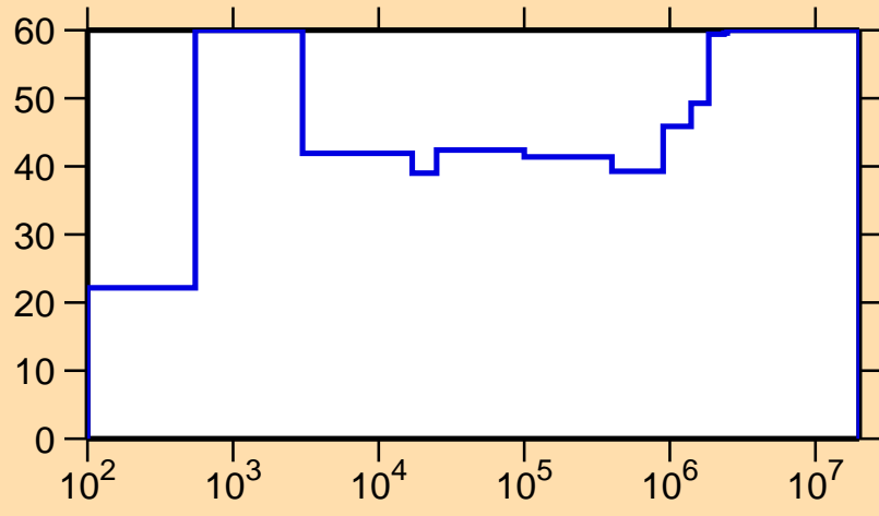
\Delta\sigma/\sigma vs. E for ^{147}\text{Gd}(n,\gamma)
