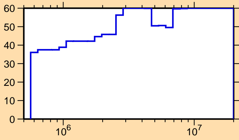
\Delta\sigma/\sigma vs. E for ^{148}\text{Gd}(n,\gamma)
