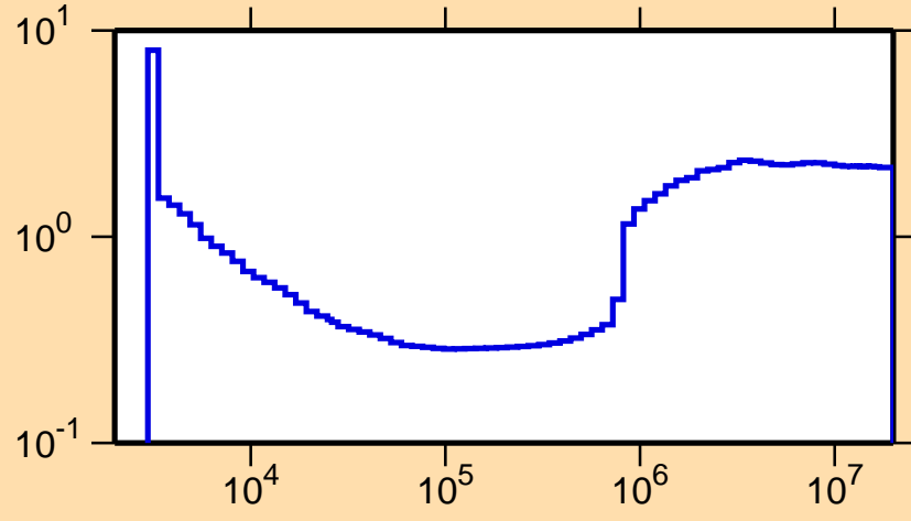
\sigma vs. E for ^{148}\text{Gd}(n,\text{nonel.})
