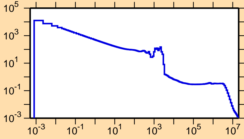
\sigma vs. E for ^{148}\text{Gd}(n,\gamma)
