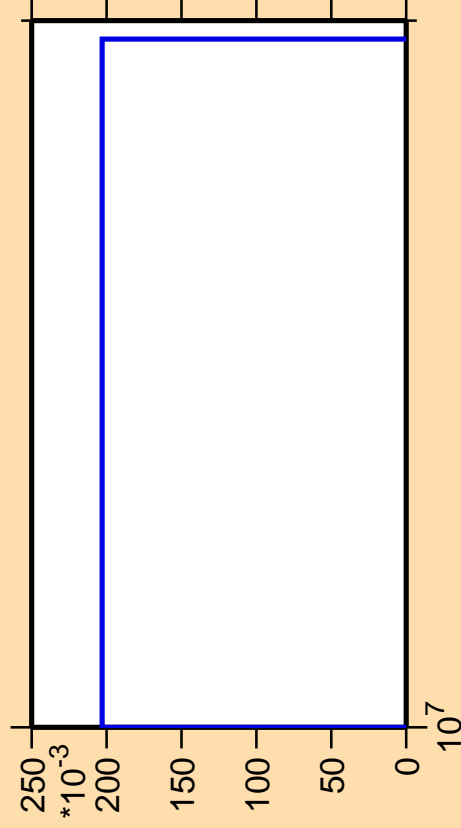
\Delta\sigma/\sigma vs. E for ^{148}\text{Gd} (mt 34)
