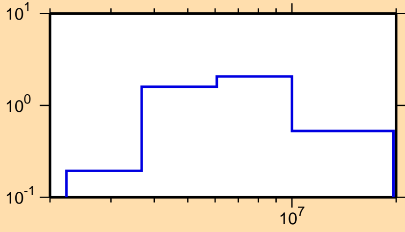
\sigma vs. E for ^{148}\text{Gd}(n,n\text{cont.})
