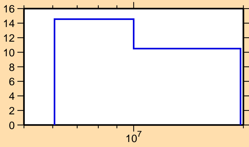
\Delta\sigma/\sigma vs. E for ^{148}\text{Gd}(n,\text{el.})
