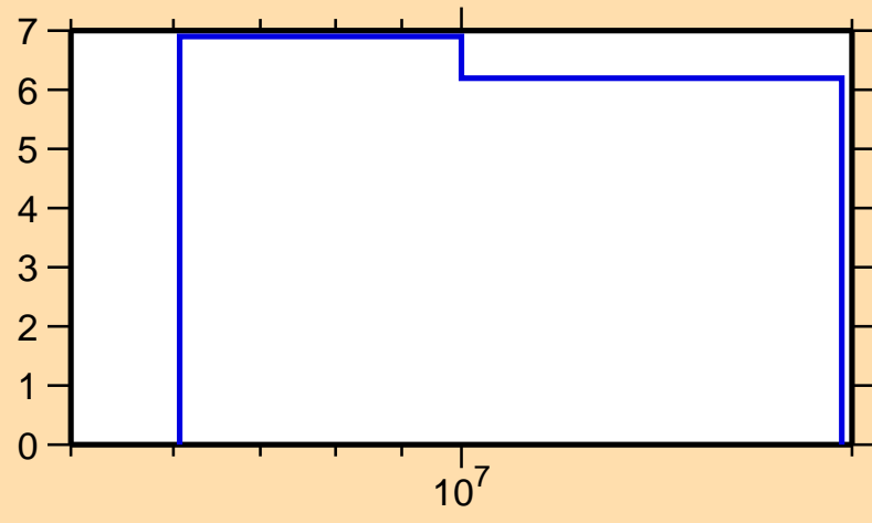
\Delta\sigma/\sigma vs. E for ^{148}\text{Gd}(n,\text{nonel.})
