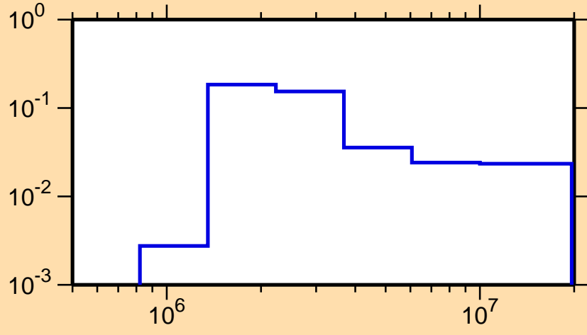
\sigma vs. E for ^{148}\text{Gd}(n,n_2)
