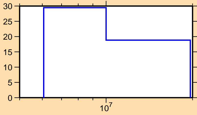
\Delta\sigma/\sigma vs. E for ^{148}\text{Gd}(n,2n)
