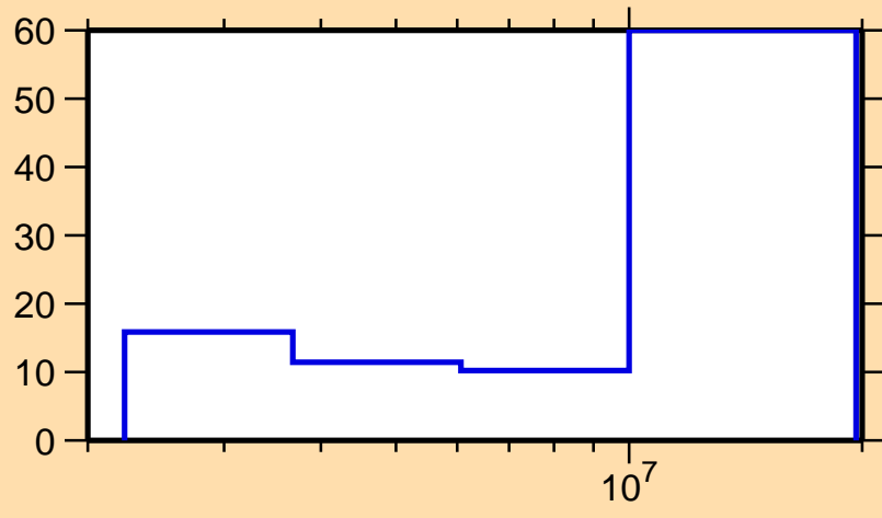
\Delta\sigma/\sigma vs. E for ^{148}\text{Gd}(n,n\text{cont.})
