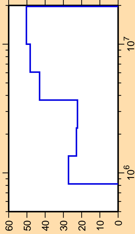
\Delta\sigma/\sigma vs. E for ^{148}\text{Gd}(n,n_2)
