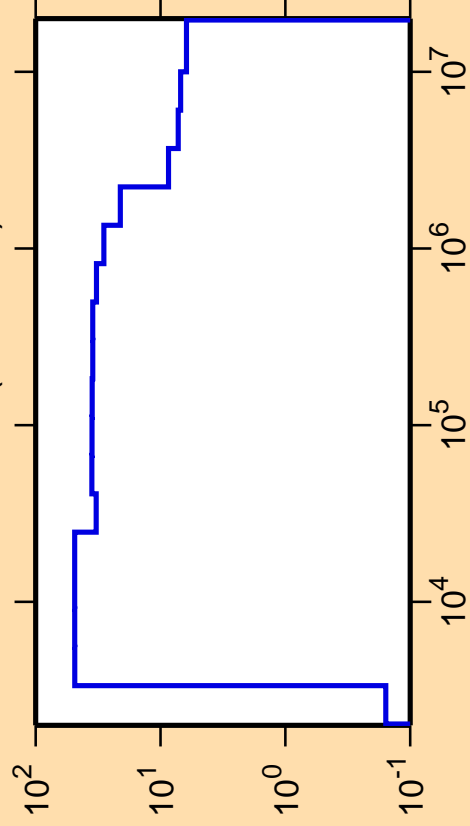
\Delta\sigma/\sigma vs. E for ^{148}\text{Gd}(n,\text{nonel.})
