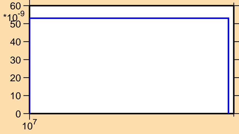
\sigma vs. E for ^{148}\text{Gd}(n,2np)
