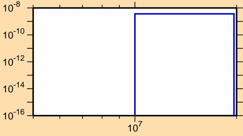
\sigma vs. E for ^{148}\text{Gd}(\text{mt117})
