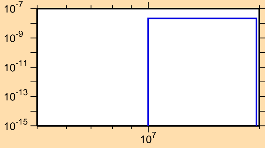
\sigma vs. E for ^{148}\text{Gd} (mt 45)
