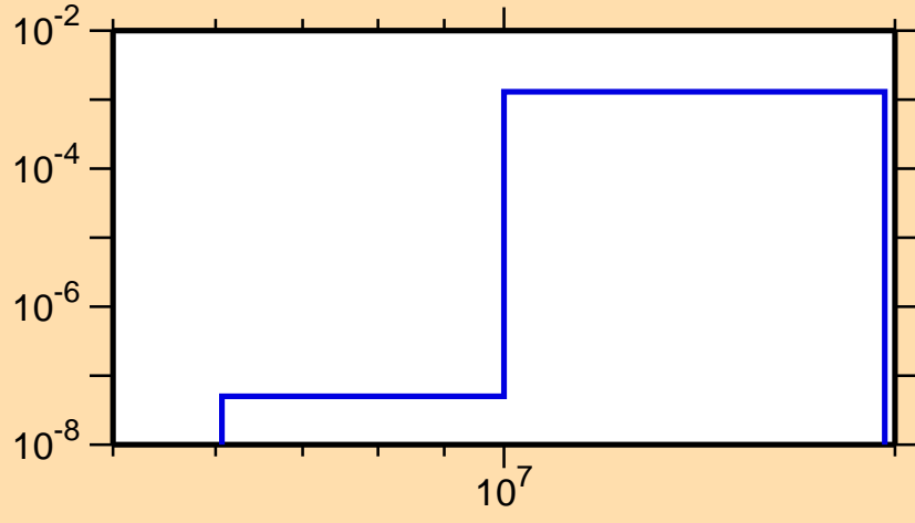
\sigma vs. E for ^{148}\text{Gd}(n,d)
