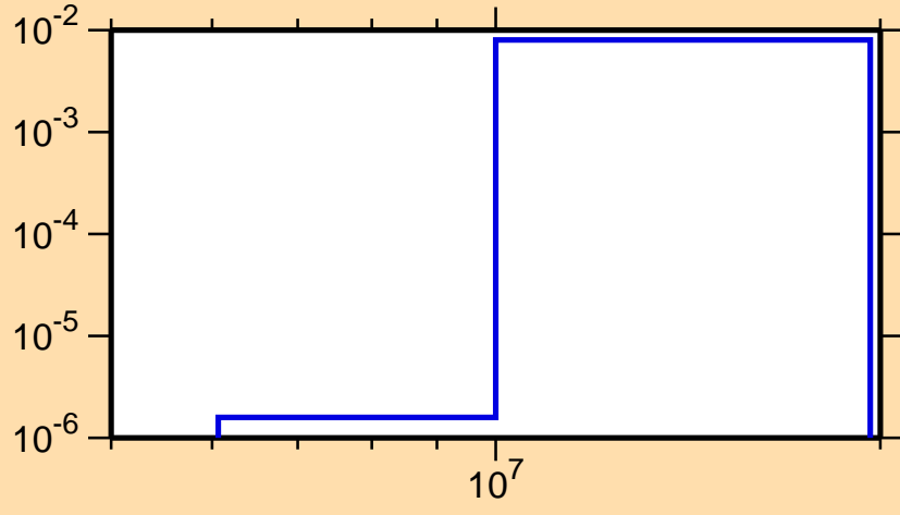
\sigma vs. E for ^{148}\text{Gd}(n,np)
