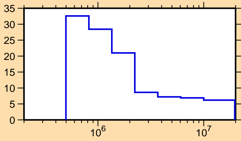
\Delta\sigma/\sigma vs. E for ^{148}\text{Gd}(n,\text{nonel.})
