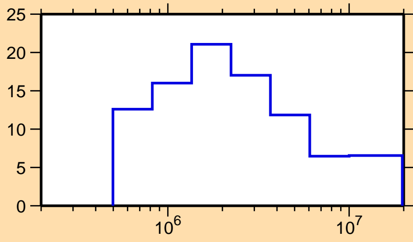
\Delta\sigma/\sigma vs. E for ^{148}\text{Gd}(n,\text{tot.})
