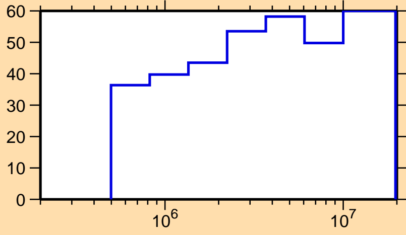
\Delta\sigma/\sigma vs. E for ^{148}\text{Gd}(n,\gamma)
