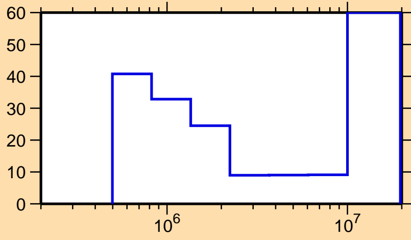
\Delta\sigma/\sigma vs. E for ^{148}\text{Gd}(n,\text{inel.})
