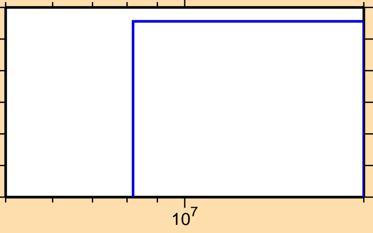
\sigma vs. E for ^{148}\text{Gd}(n,2np)
