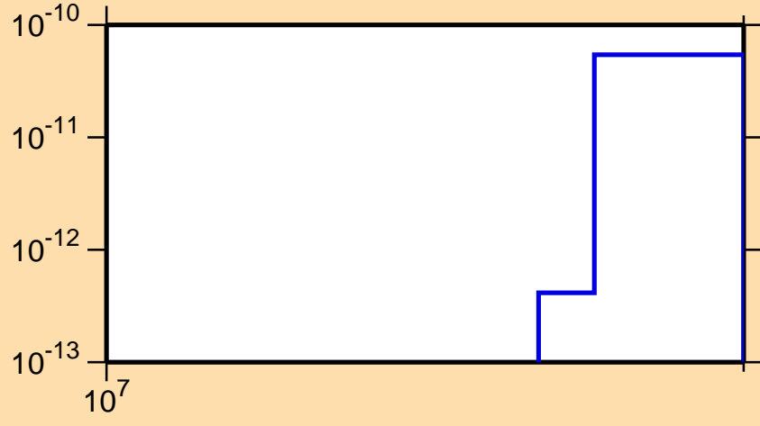
\sigma vs. E for ^{149}\text{Gd} (mt 34)
