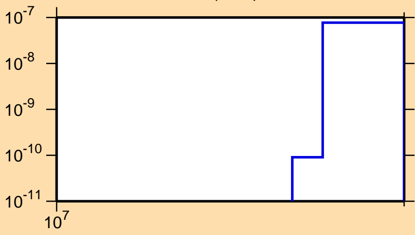
\sigma vs. E for ^{149}\text{Gd}(n,nt)
