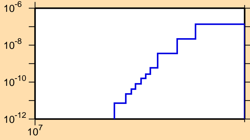
\sigma vs. E for ^{149}\text{Gd}(\text{mt } 45)
