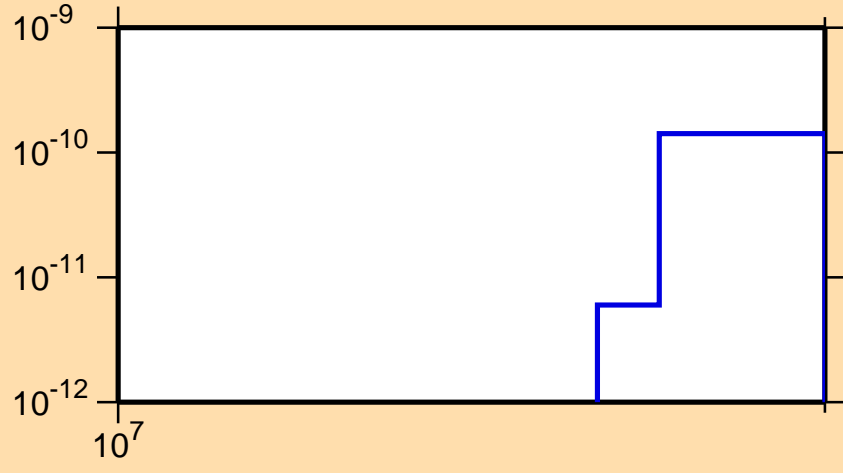
\sigma vs. E for ^{149}\text{Gd}(n,\text{pd})
