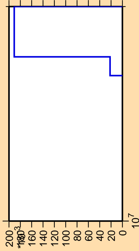
\Delta\sigma/\sigma vs. E for ^{149}\text{Gd}(n,3n\alpha)
