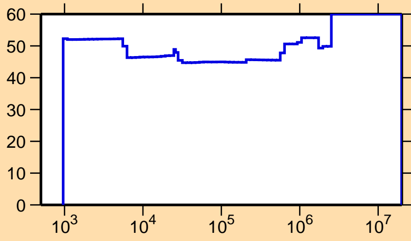
\Delta\sigma/\sigma vs. E for ^{149}\text{Gd}(n,\gamma)
