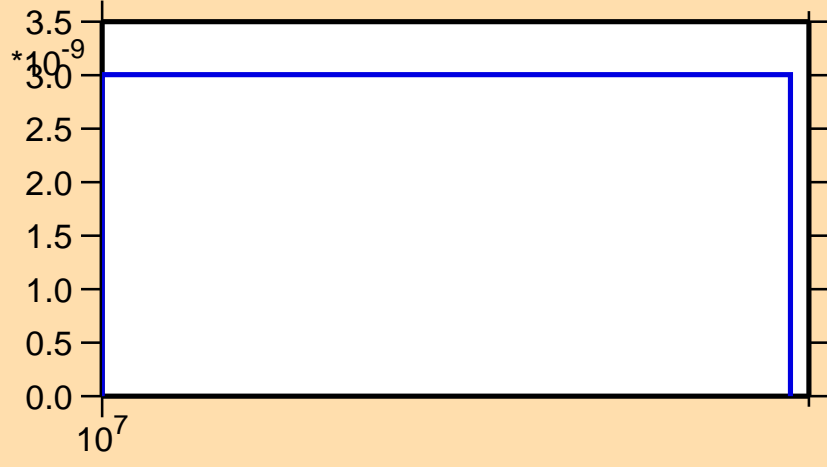
\sigma vs. E for ^{149}\text{Gd} (mt 45)
