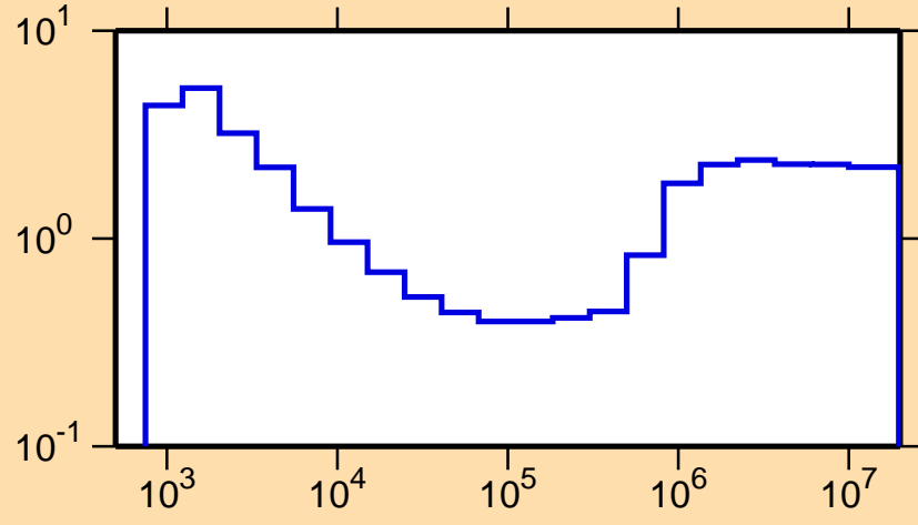
\sigma vs. E for ^{150}\text{Gd}(n,\text{nonel.})
