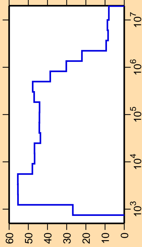
\Delta\sigma/\sigma vs. E for ^{150}\text{Gd}(n,\text{nonel.})
