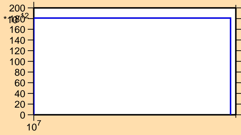
\sigma vs. E for ^{150}\text{Gd}(n,nt)
