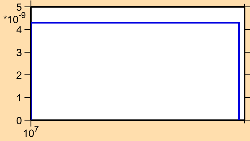
\sigma vs. E for ^{150}\text{Gd}(n,nd)
