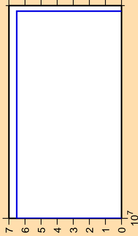
\Delta\sigma/\sigma vs. E for ^{150}\text{Gd}(n,\text{pd})
