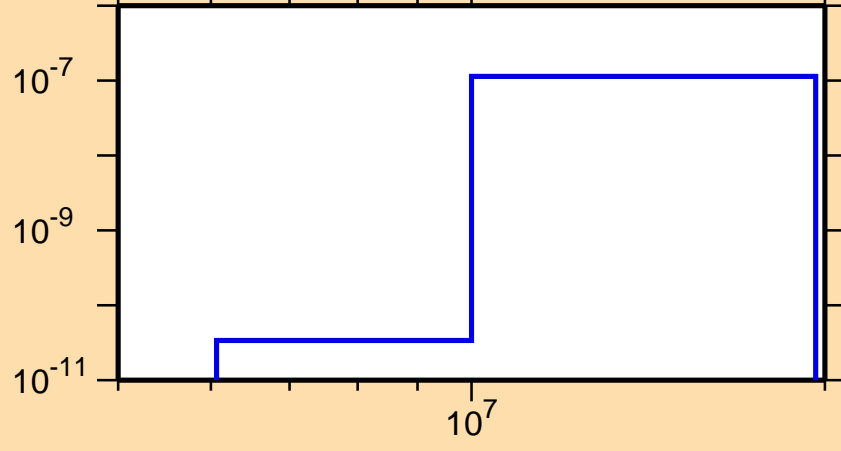
\sigma vs. E for ^{150}\text{Gd}(n,p\alpha)
