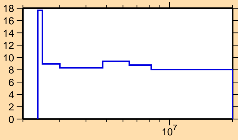
\Delta\sigma/\sigma vs. E for ^{150}\text{Gd}(n,n\text{onel.})
