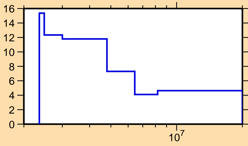
\Delta\sigma/\sigma vs. E for ^{150}\text{Gd}(n,\text{tot.})
