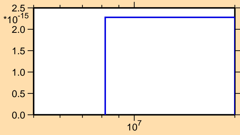
\sigma vs. E for ^{150}\text{Gd} (mt 34)
