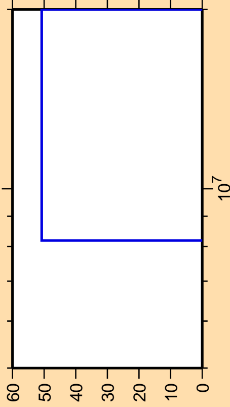
\Delta\sigma/\sigma vs. E for ^{150}\text{Gd}(n,n_1)
