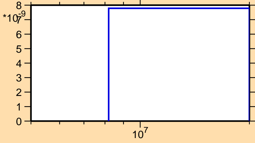
\sigma vs. E for ^{150}\text{Gd}(n,\text{He3})
