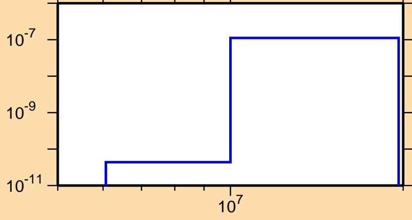
\sigma vs. E for ^{151}\text{Gd}(n,p\alpha)
