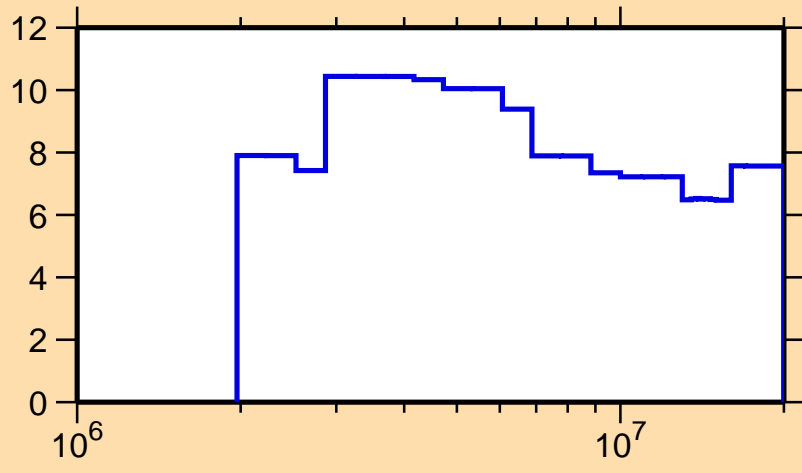
\Delta\sigma/\sigma vs. E for ^{152}\text{Gd}(n,n\text{onel.})
