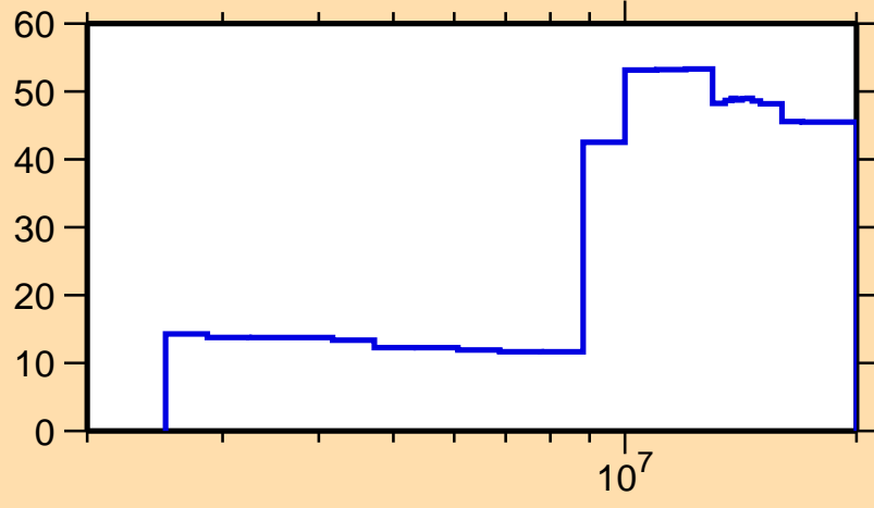
\Delta\sigma/\sigma vs. E for ^{152}\text{Gd}(n,n\text{cont.})
