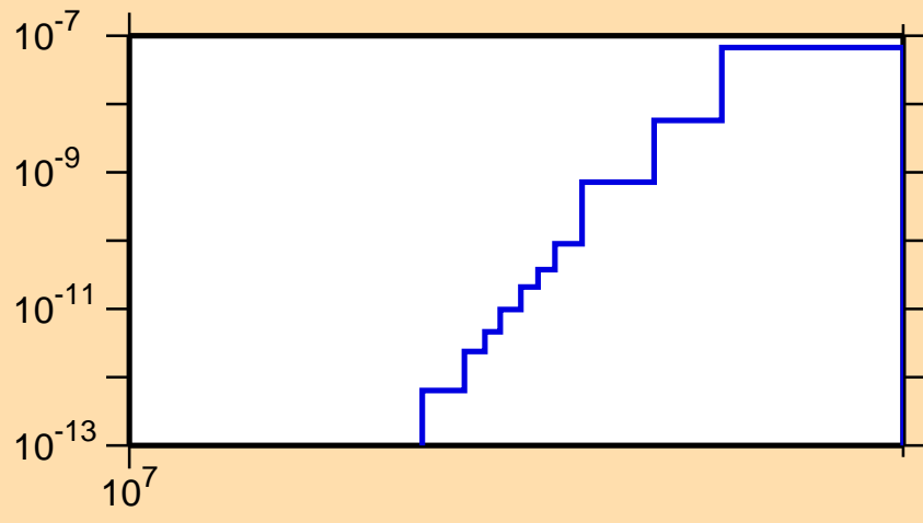
\sigma vs. E for ^{152}\text{Gd}(n,\text{He3})
