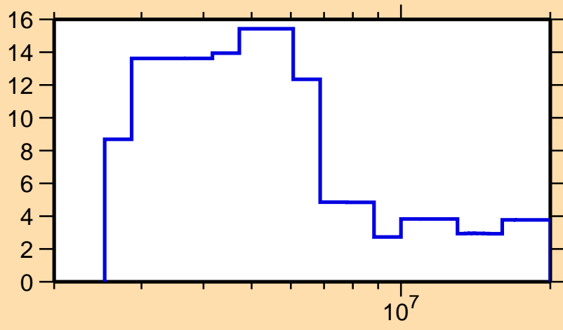
\Delta\sigma/\sigma vs. E for ^{152}\text{Gd}(n,\text{tot.})
