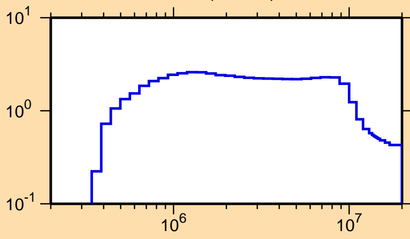
\sigma vs. E for ^{152}\text{Gd}(n,\text{inel.})
