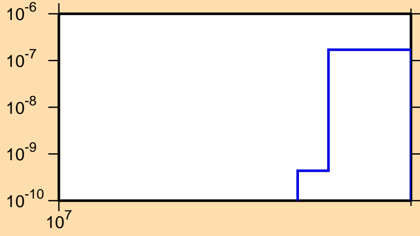
\sigma vs. E for ^{152}\text{Gd}(n,\text{nd})
