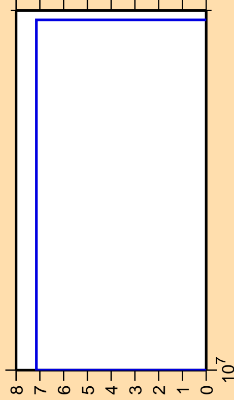
\Delta\sigma/\sigma vs. E for ^{152}\text{Gd}(\text{mt117})
